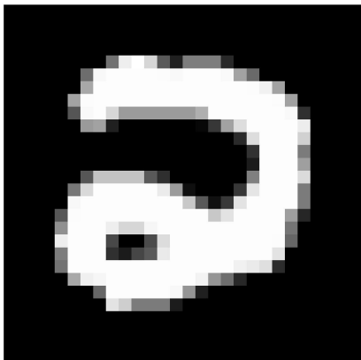
Reconstruction MSE: 0.1225
