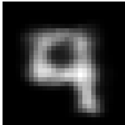
Reconstruction MSE: 0.1123
