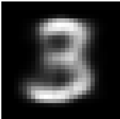
Reconstruction MSE: 0.1171
