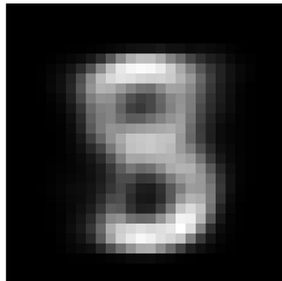
Reconstruction MSE: 0.1039
