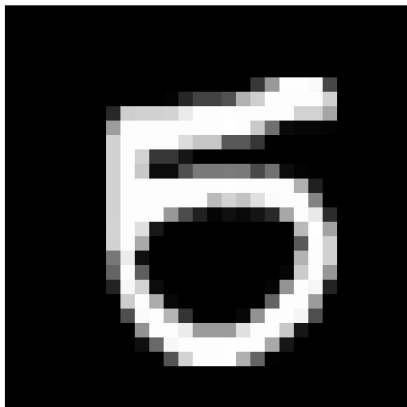
Reconstruction MSE: 0.1143
